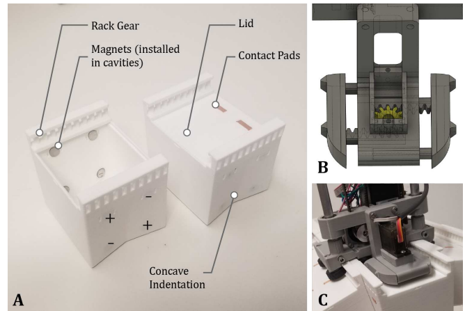
Fig. 3. (A) The blocks used in the demonstration measure roughly 50 \text{ mm} \times 68 \text{ mm} \times 57 \text{ mm} and are 3D printed with embedded features like rack gears to facilitate robot locomotion, shaped faces to facilitate alignment and enhance structural stability, a channel to hold a lid, and cavities to mount magnets. Magnets are installed in a pattern of alternating polarity (the same pattern is mirrored on the reverse side). (B) Detail of the RailBot's gripper with the motor removed, showing the pairwise rack-and-pinion mechanism. (C) Detail of the robot's gripper, having just retracted after placing a block.
