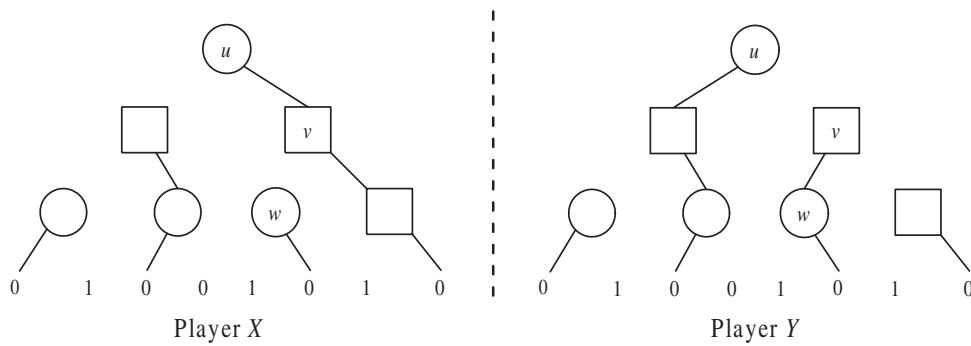
FIG. 2. An illustration of the compression protocol for nonproduct distributions. The circle nodes are owned by player X and the square nodes are owned by Y . The figure illustrates the states of the protocol trees after all the bits have been sampled. The players then proceed to resolve their disagreements. The disagreement at node u is resolved in favor of X since he owns the node. The protocol proceeds to node v where the disagreement is resolved in favor of Y . The final computation path in this case is u - v - w , the output is 0, and the total number of disagreements along the path is 2.
