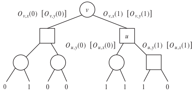
FIG. 1. An illustration of the protocol tree for \pi . The round nodes are owned by X and the square nodes are owned by Y . On each edge the “correct” probability is indicated. The “approximate” probability that is estimated by the player who does not own the node is shown in the brackets.
