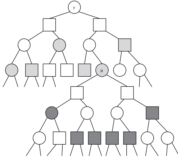
FIG. 3. An illustration of the compression protocol for product distributions. The gray layer represents the “frontier” of nodes where some fixed amount of information is conveyed in the original protocol, and which is simulated in one iteration of the compressed protocol. Once the players agree on a node u , they compute a new frontier, illustrated here by the black layer.
