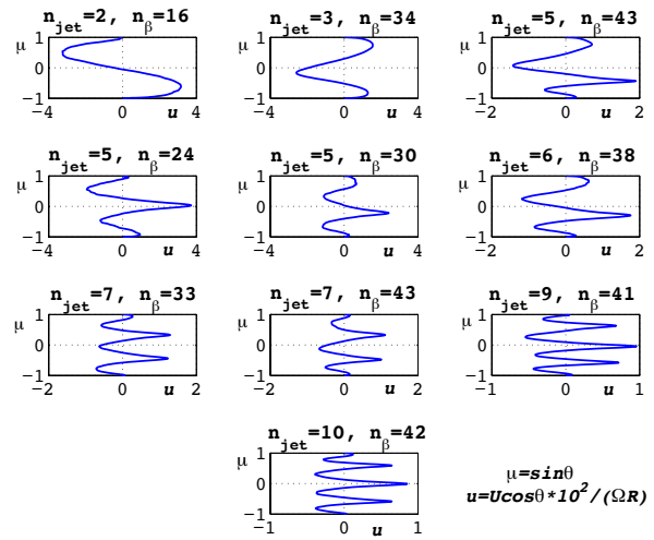
Fig. 9. Zonal velocity profiles for different combinations of n_{\text{jet}} and n_{\beta} from various long-term simulations using 2-D vorticity equation on the surface of a rotating sphere.
