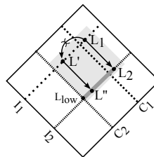
Fig. 11: Bounded endorsement and robust declassification.
