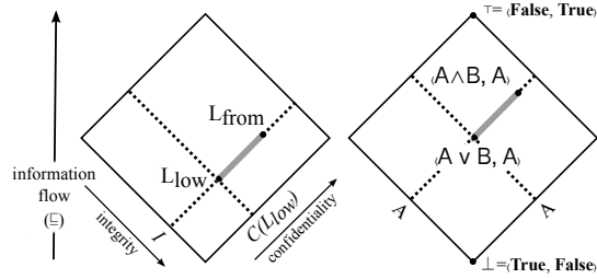
Fig. 8: Robust Declassification
