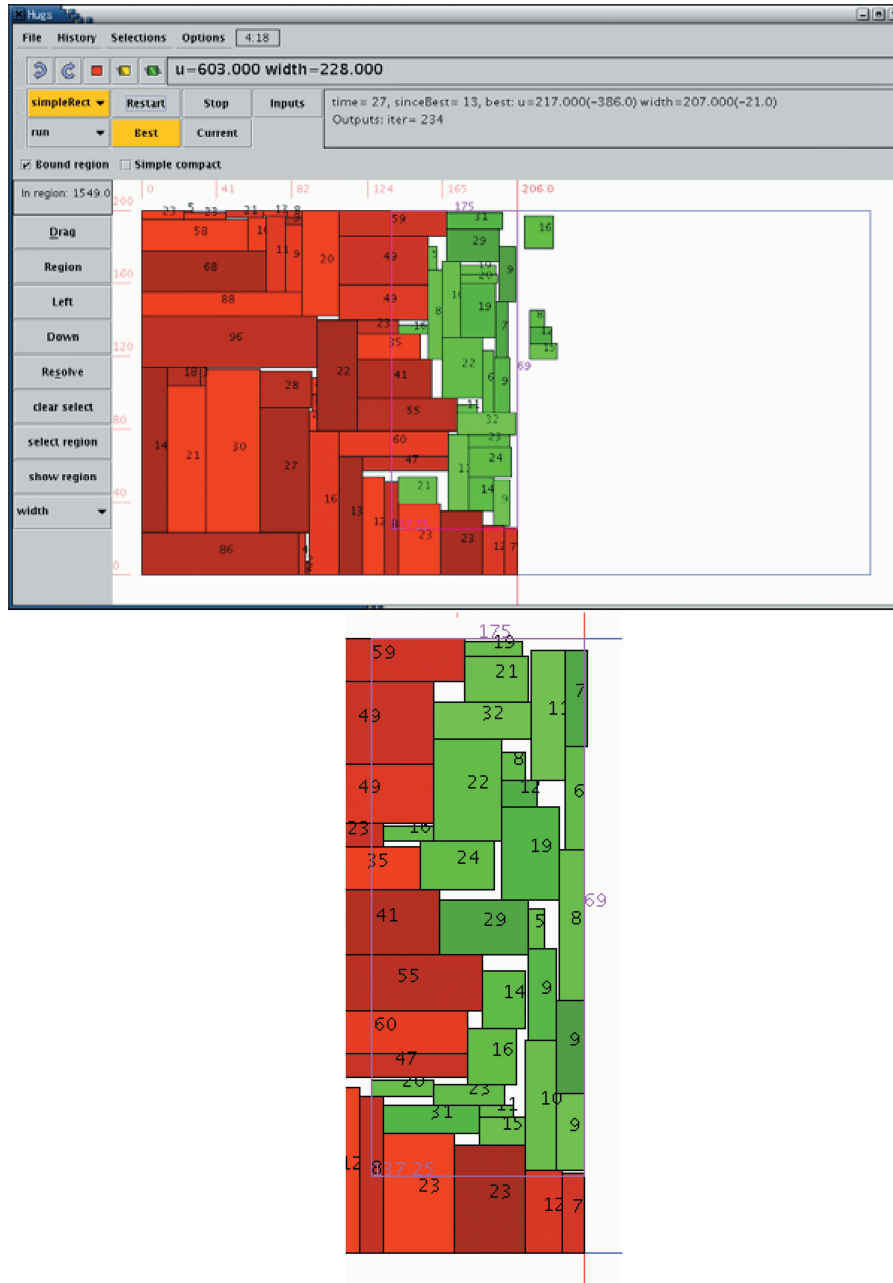
Fig. 2. Interactive system: The top image is a screen shot of our system in use. The user has selected a region to apply BLD* to and has frozen most of the rectangles (frozen rectangles shown in red/dark gray, unfrozen in green/light gray). The image on the right shows a blowup of the selected portion on the packing, after BLD* has run for a few seconds and the user has pressed the Best button to see the best solution found.
