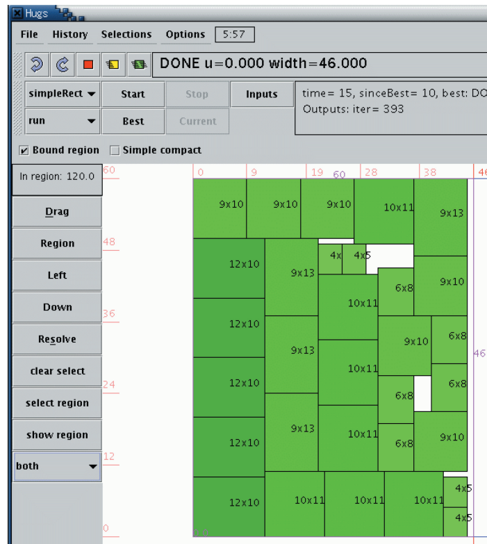
Fig. 3. Our solution to the D1 dataset, which is one unit better than the best previously published solution. The solution has width 46 in our interface, or height 46 in the standard formulation.
