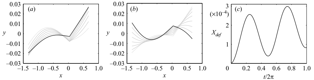
FIGURE 12. (a) Thrust, (b) recovery. M_n = 1.0 , \Omega = 80 , b_0 = 0.5 and N_p = 81 . The transverse field b_0 \sin t decreases from b_0 to -b_0 over the half-cycle. The dotted line represents the initial shape, the solid line the final shape, and grey lines intermediate shapes. The remaining half of the cycle can be obtained by mirror reflection in the x -axis. (c) x -displacement of the defect during the stroke sequence.
