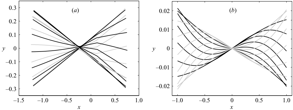
FIGURE 11. (a) Kinematics of the swimming stroke at low ( M_n = 1.0 , \Omega = 2.0 ) frequency. The defect is located at s^* = 0.32 . (b) Stroke of filament at \Omega = 80 without defect for contrast with figure 12(a, b). As a visual aid, the cycle is split into two halves: defect point moving in the negative y -direction (black curves), and defect point moving in the positive y -direction (grey curves) Both simulations are performed with b_0 = 0.5 and N_p = 81 .
