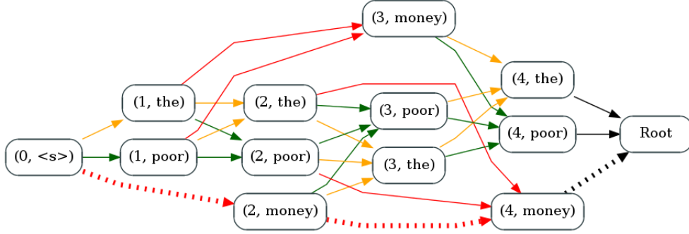
Figure 2: Hypergraph for translating the sentence w = \text{les}_1 \text{pauvres}_2 \text{sont}_3 \text{demunis}_4 with set of pairs \mathcal{P} = \{(\text{les}, \text{the}), (\text{pauvres}, \text{poor}), (\text{sont demunis}, \text{don't have any money})\} . Hyperedges are color-coded by source words translated: orange for \text{les}_1 , green for \text{pauvres}_2 , and red for \text{sont}_3 \text{demunis}_4 . The dotted lines show an invalid hyperpath x that has signature Ax = \langle 0, 0, 2, 2 \rangle \neq \langle 1, 1, 1, 1 \rangle .
